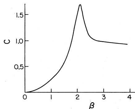
FIG. 2. The specific heat C vs \beta=4/g^2 for an SU(2) lattice gauge theory, taken from the Monte Carlo study of Ref. 25. The values of C on the curve are accurate only to within an error of roughly 5 to 10%.
